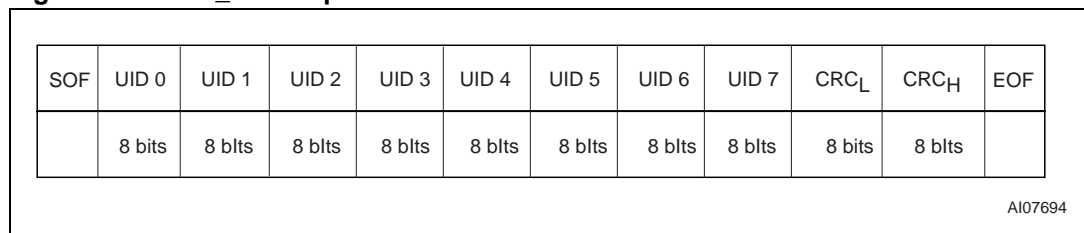
Figure 46. GET_UID response format
