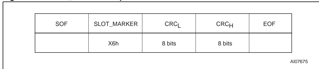
Figure 27. SLOT_MARKER request format
