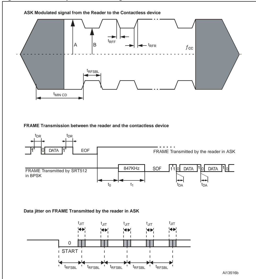
Figure 49. SRT512 synchronous timing, transmit and receive
