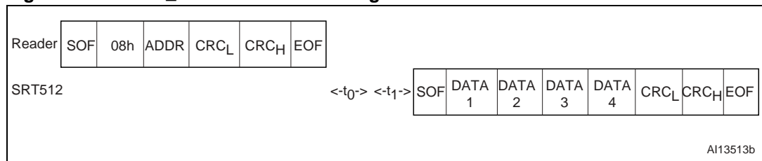
Figure 41. READ_BLOCK frame exchange between Reader and SRT512
