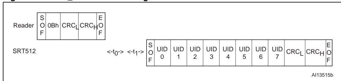
Figure 61. GET_UID frame exchange between Reader and SRT512
