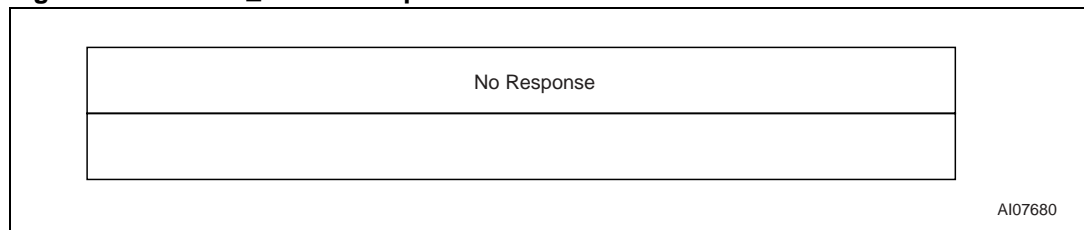
Figure 43. WRITE_BLOCK response format
