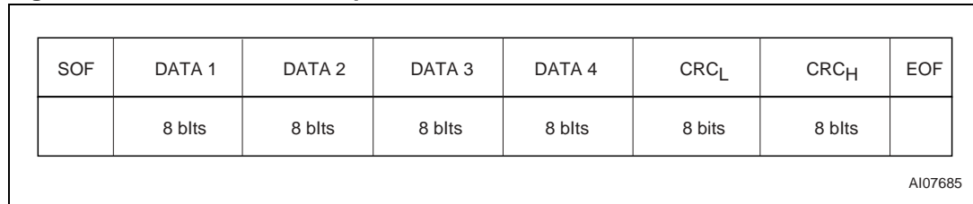
Figure 40. READ_BLOCK response format
