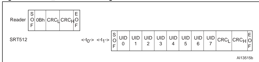
Figure 48. GET_UID frame exchange between Reader and SRT512
