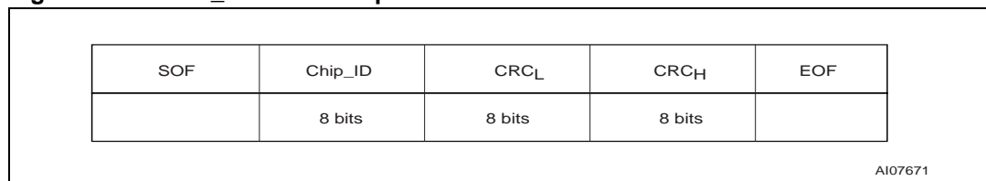
Figure 28. SLOT_MARKER response format
