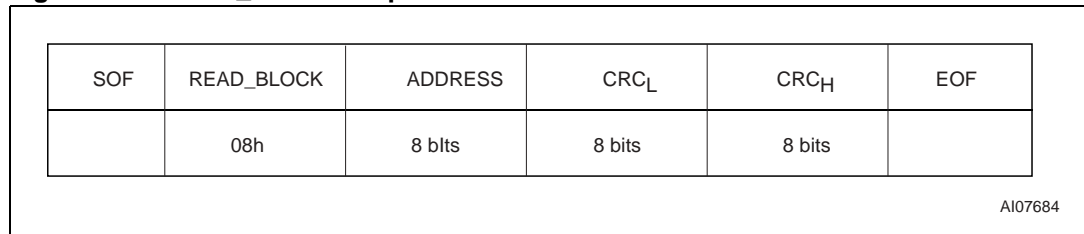
Figure 39. READ_BLOCK request format
