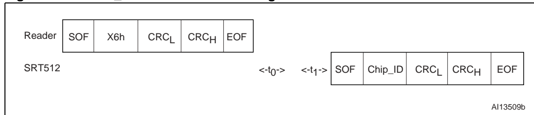
Figure 29. SLOT_MARKER frame exchange between Reader and SRT512
