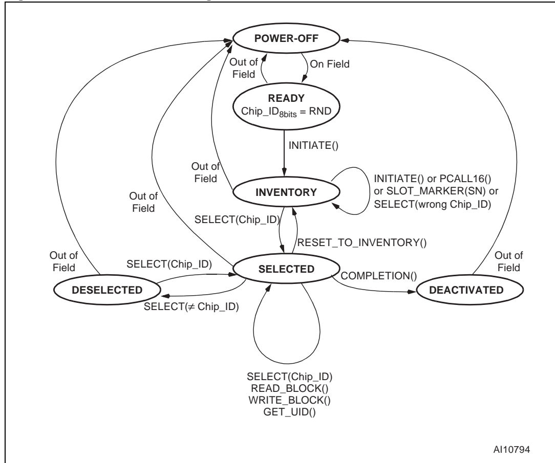
Figure 17. State transition diagram
