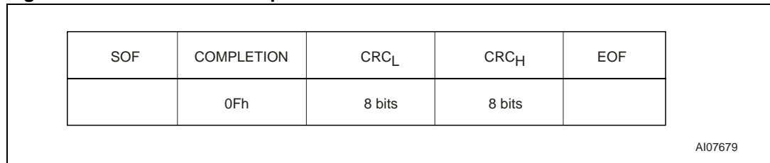
Figure 33. COMPLETION request format
