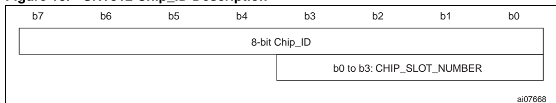
Figure 18. SRT512 Chip_ID Description
