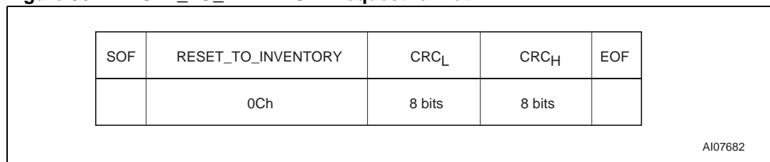
Figure 36. RESET_TO_INVENTORY request format
