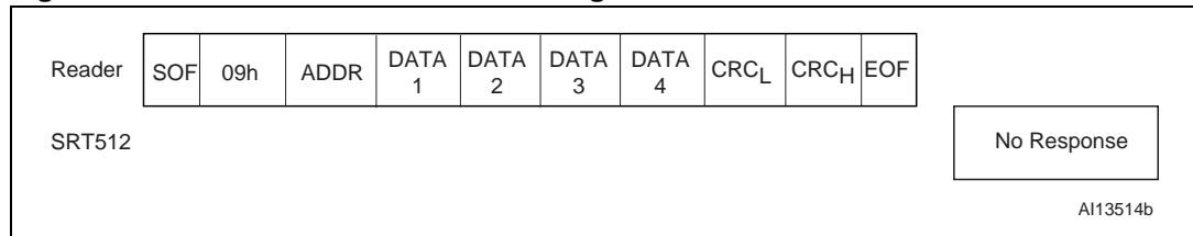
Figure 44. WRITE_BLOCK frame exchange between Reader and SRT512
