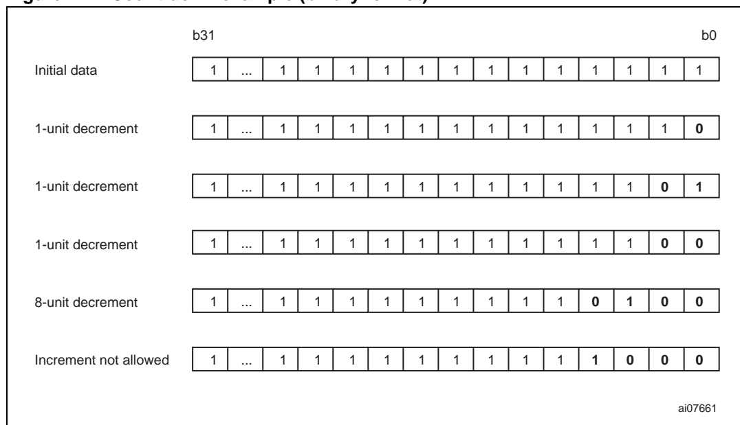
Figure 14. Count down example (binary format)
