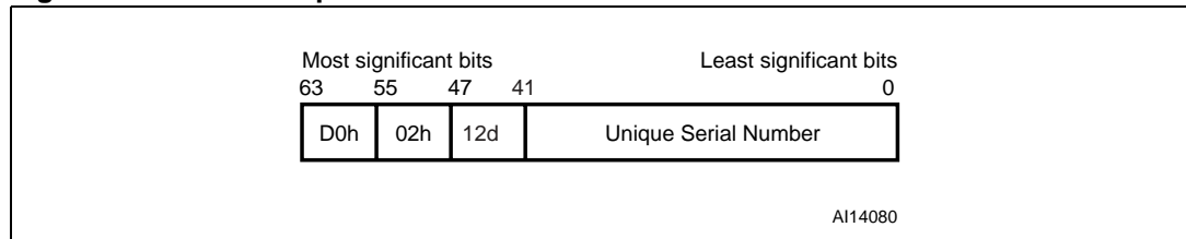
Figure 47. 64-bit unique identifier of SRT512
