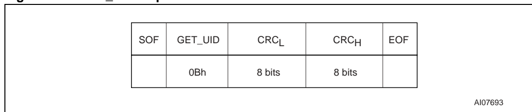
Figure 45. GET_UID request format
